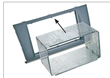
Place the Double-DIN facia plate at the dashboard, move metal bracket into the facia plate.
